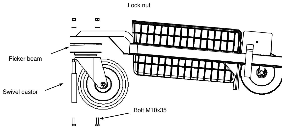
Figure 9: Assembly, step 3
