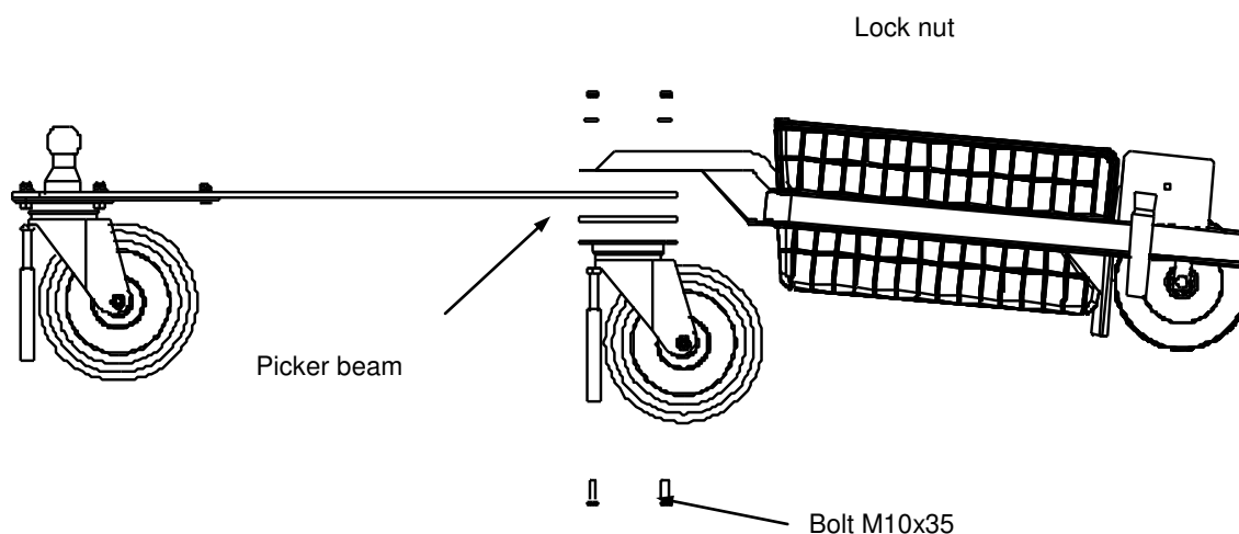
Figure 8: Assembly, step 2
