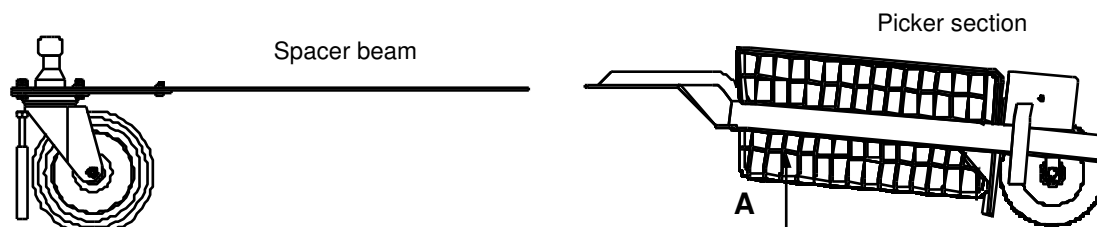
Figure 7: Assembly, step 1
